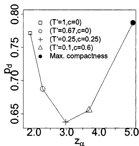
FIG. 10. The relationship of p_d and z_\alpha = n_\alpha/n for self-avoiding walks generated using different (T', c) parameters at chain length 1800.
