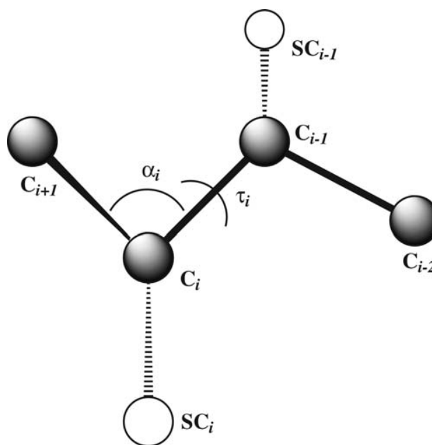
Fig. 1. Discrete state model for protein structures. Bond angle \alpha_i at position i is formed by C_{i-1} , C_i and C_{i+1} . Torsion angle \tau_i is the dihedral angle of the two planes formed by atoms (C_{i-2}, C_{i-1}, C_i) and (C_{i-1}, C_i, C_{i+1}) .
