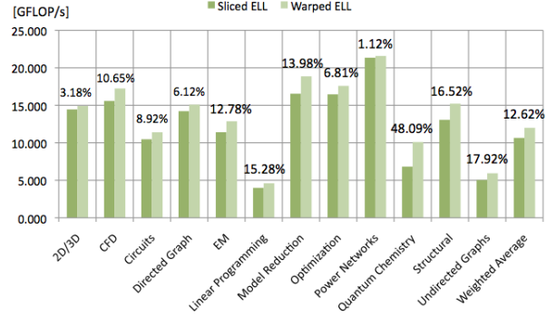
Figure 5. Sliced ELL versus Warp-grained sliced ELL
