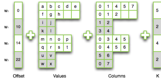
Figure 4. Sliced ELL with warp granularity
