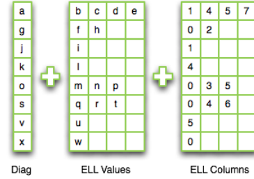
(b) ELL with separate diagonal
